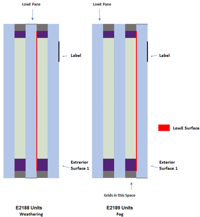
Figure 2 – Low E Surface for Triple Glazed Units
